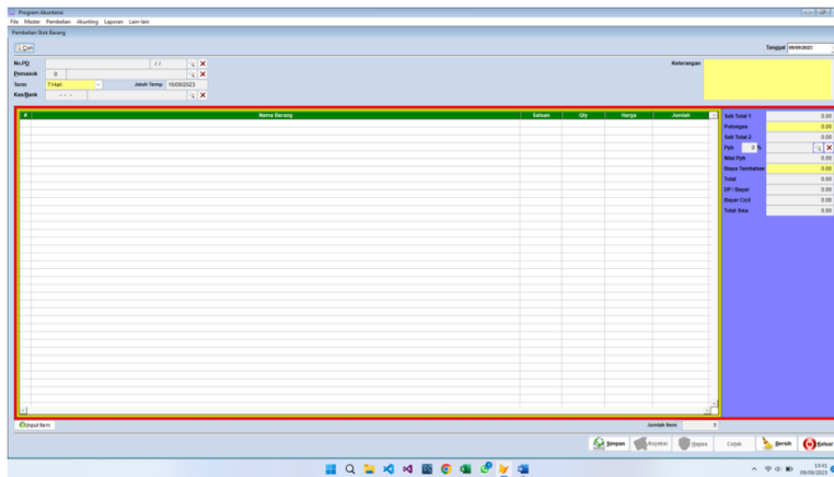
Gambar 5. Menu Utilities
